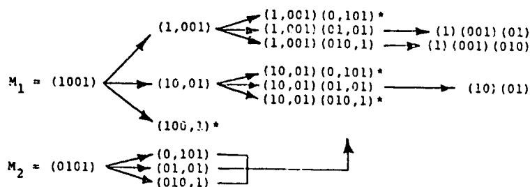
Figure 10. ALL PERMISSIBLE SEGMENTATIONS OF TWO MESSAGES INTO TWO WORDS BY APPLYING THE RULE OF PRIMITIVE EXTENSIONS.
